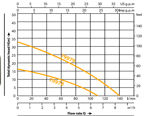
PERFORMANCE CURVE
